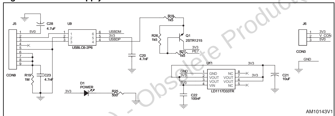
Figure 6. Power supply
