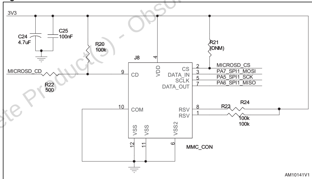
Figure 4. MicroSD
