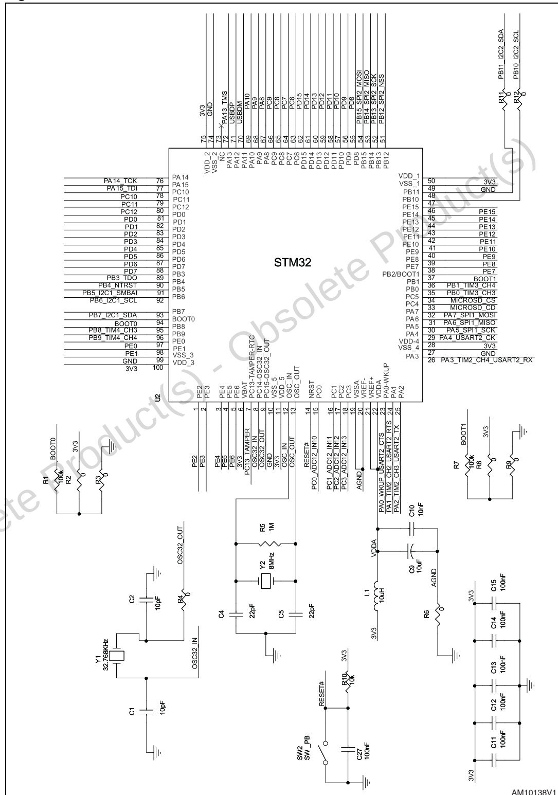
Figure 1. Microcontroller
